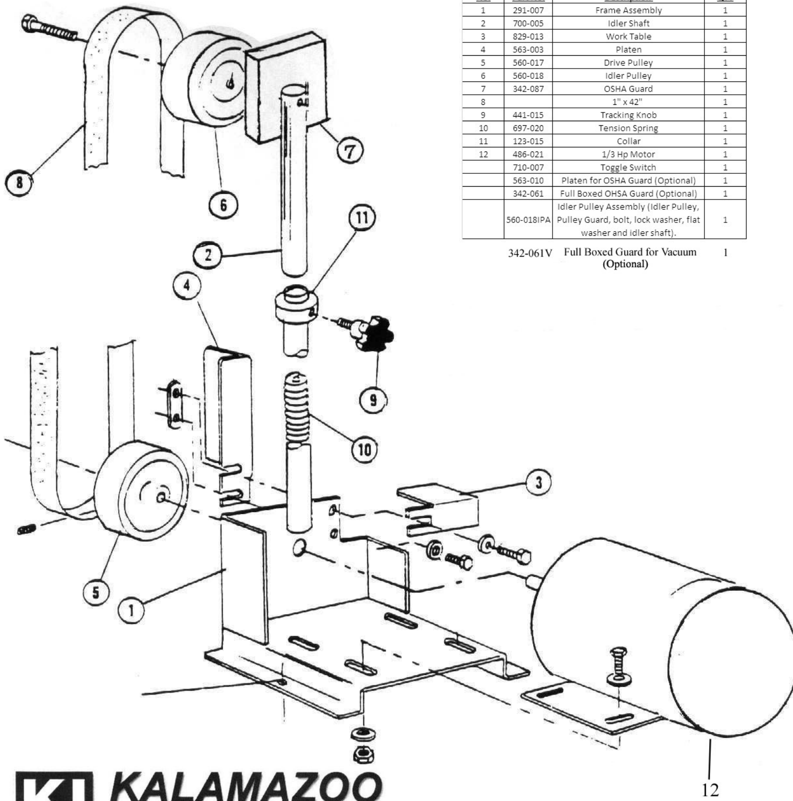
1SM Belt Sander Parts List
